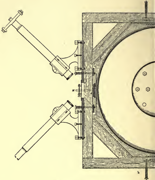
FIG. 17 Plan of optical frame with steel disk in position. C represents one of the panes of optical frame shown, and part of the fixing of the four mirrors. Each mirror held by a brass plate and it is pressed by the spring-bolts shown.
