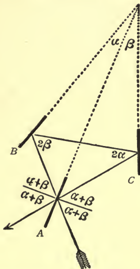
FIG. 7.—Plan of Interference Kaleidoscope with three mirrors.
