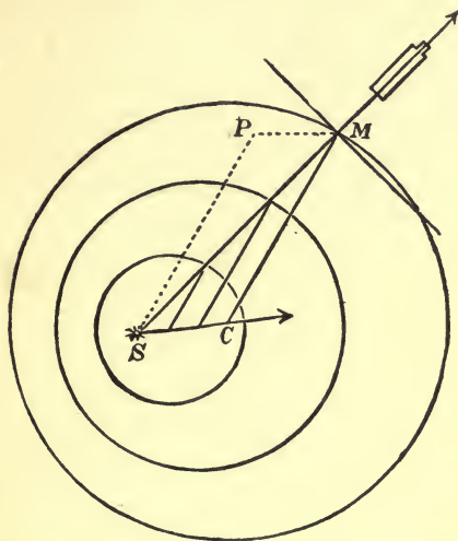
FIG. 5.—Successive Wave Fronts in a Moving Medium.
