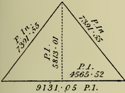
Direct Vertical Section of Gr. Pyr. d
