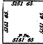
Square with side computed by \pi .
