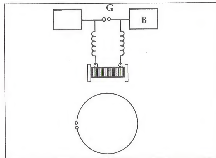
Apparatus used by Hertz to demonstrate the wave like nature of electromagnetism.
