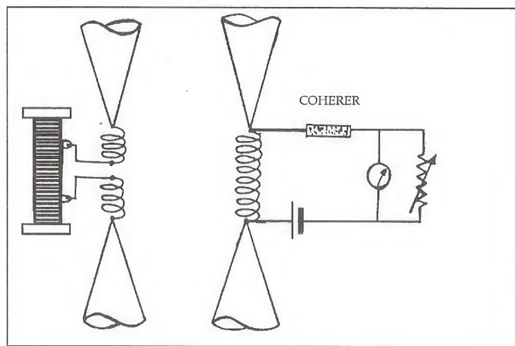
Lodge's transmitter and receiver.
