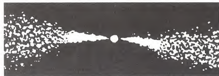
Fig. 1 Radiograph of a typical radio galaxy with jets projecting from its whirling black hole nucleus.
